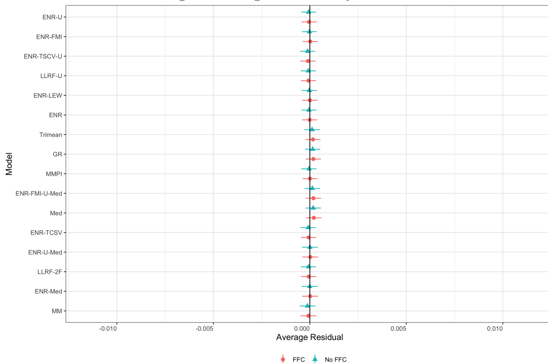
Fig. 5. Average Residual By Model
