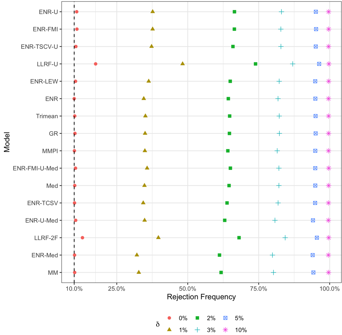
Fig. 4. Power Analysis - SQ Test
