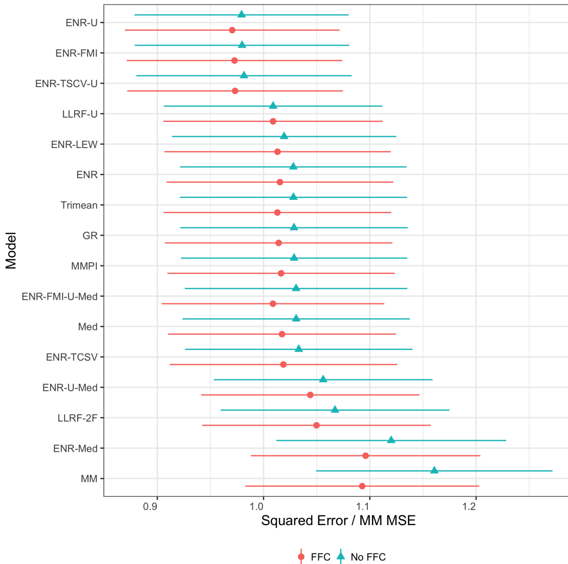
Fig. 1. Mean Squared Error By Specification: 10,000 Simulations
