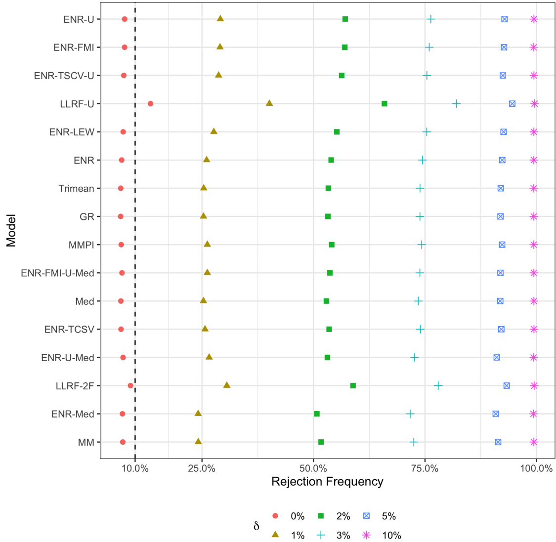
Fig. 3. Power Analysis - Standard Approach Tests of Significance
